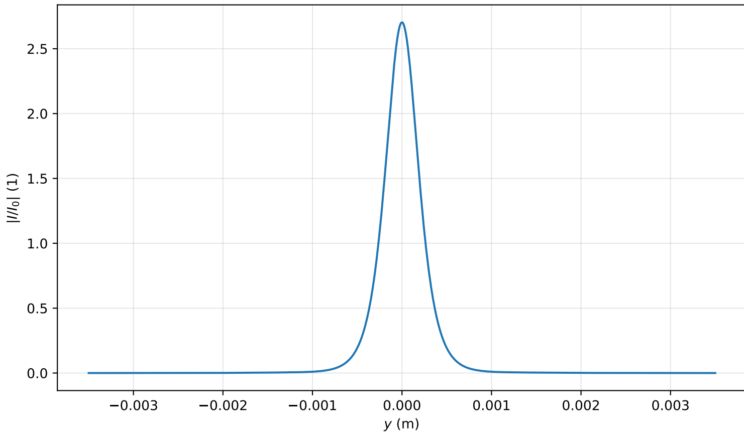
Intensity profile I(x=0, y, z=3.105)/I_0 , P_{in}=1.0P_{cr} , artificial time
